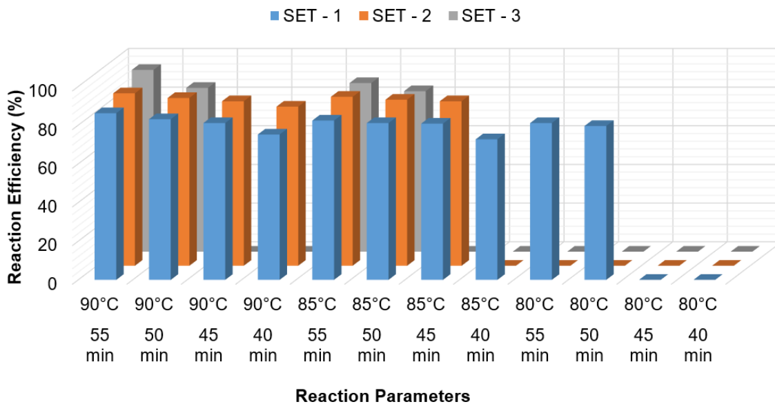
Fig. 6: The reaction efficiencies of the synthesized zinc borate compounds.
