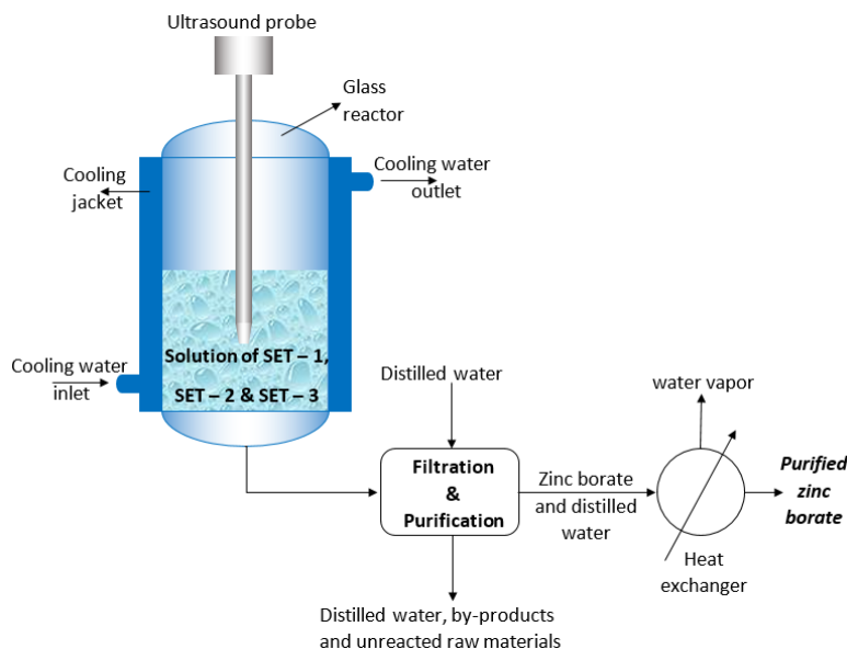
Fig. 1: Reaction procedure of zinc borate.
