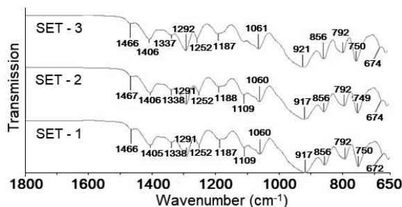
Fig. 3: FT-IR spectra of the optimum products
